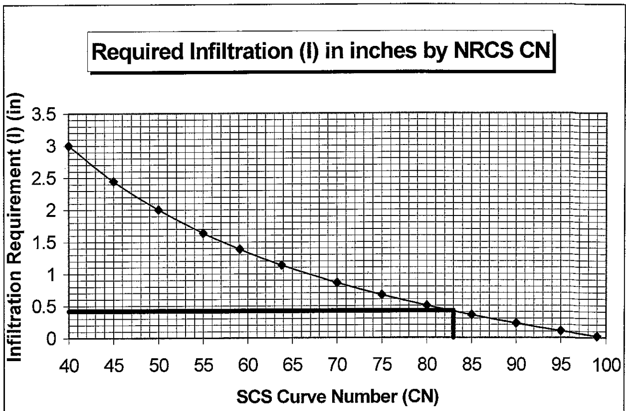
Figure 305.1. Infiltration requirement based upon NRCS Curve Number.
